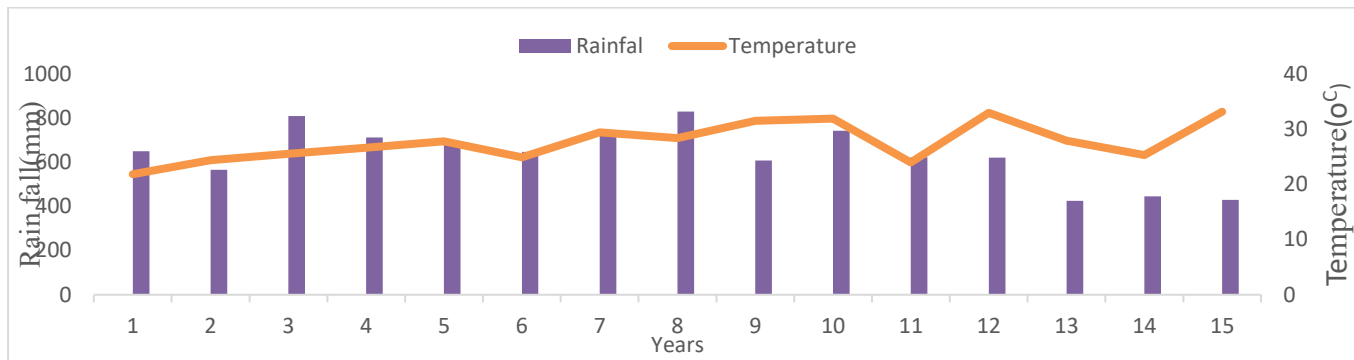
Figure 2: Mean temperature and rainfall distribution in the study area (Bishoftu Research, center institution daily-recorded data from 2003 to 2017).
